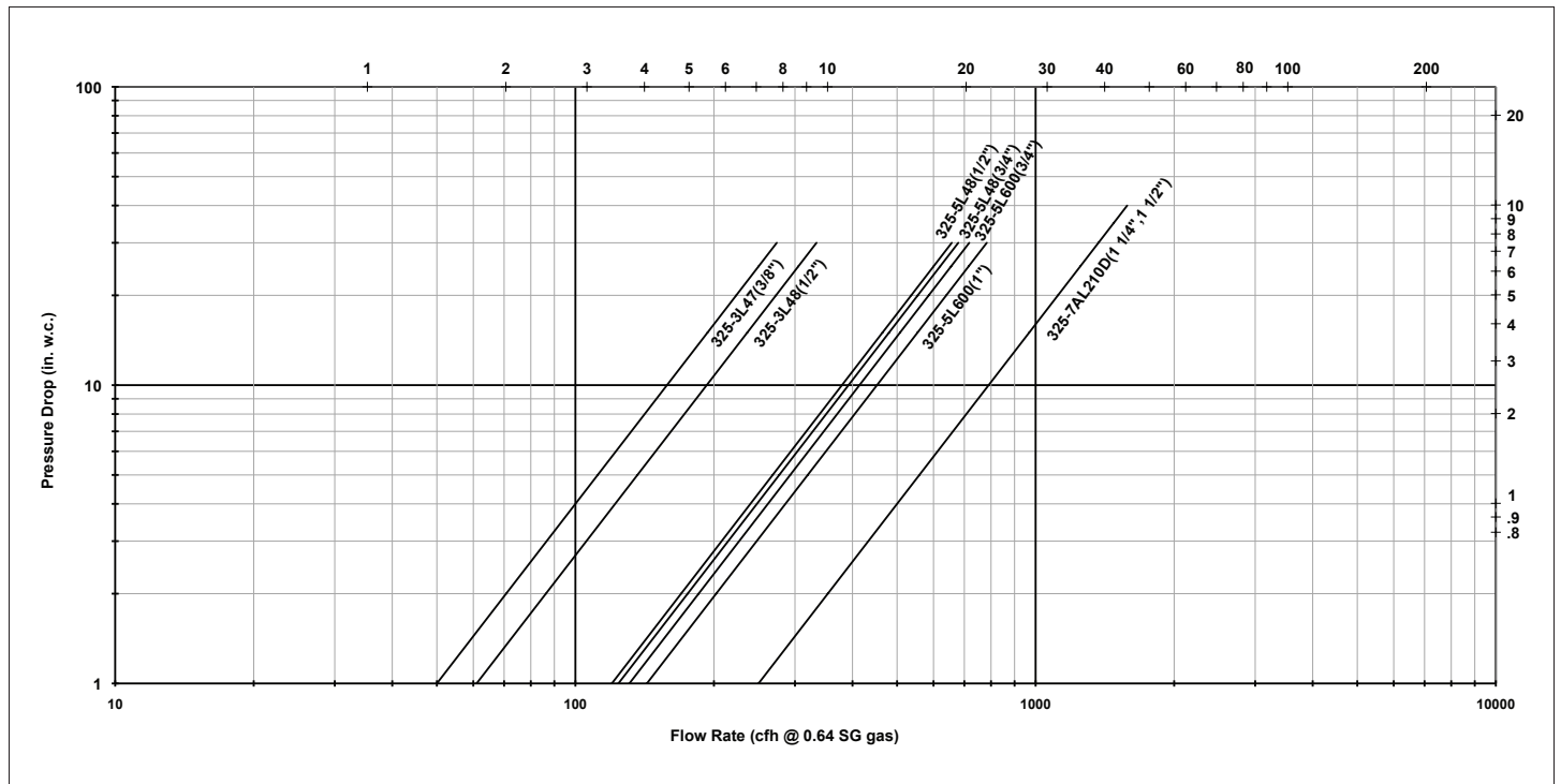
Figure 4: Pressure Drop Chart
