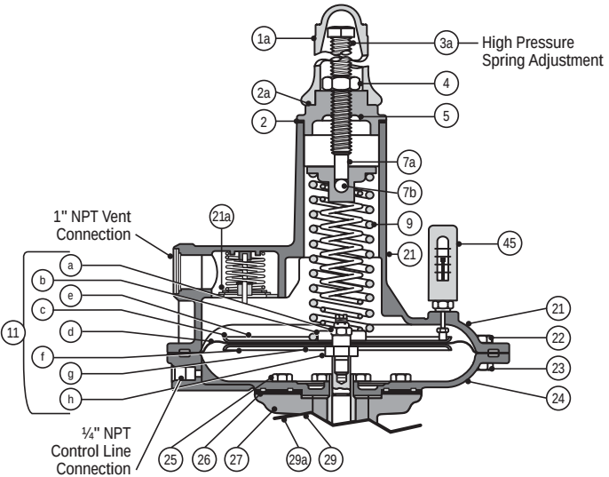
121-8 HP – HIGH PRESSURE – BACK PRESSURE
