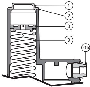
Fig. 1 Adjustment and Vent Connection 21b for Differential Regulators, Atmospheric Regulators and Zero Governors
