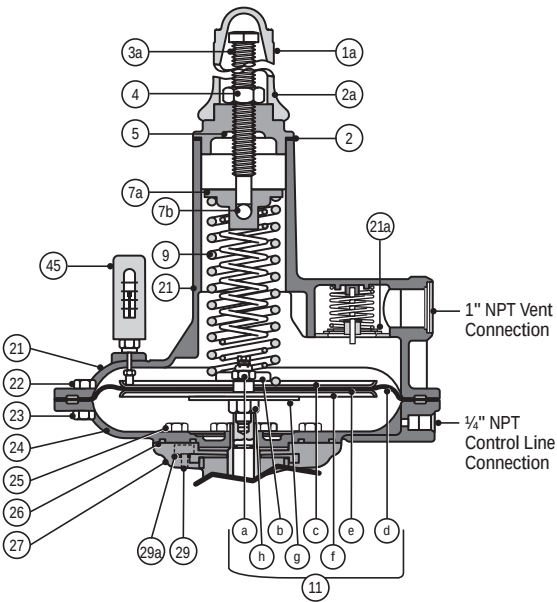
121-8 HP – HIGH PRESSURE
