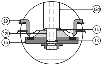
V-PORT WING OPTION
