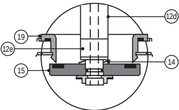
STANDARD RETAINER OPTION
